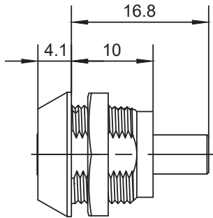
锁闭状态 Locked state
