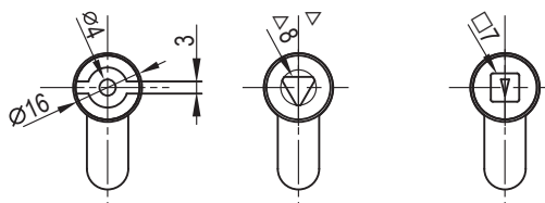
双翅 4m m Double Bit 4mm
