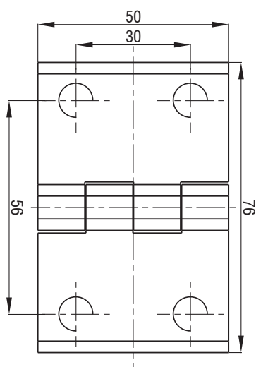
M6 镶嵌螺柱 With Threaded Studs M6
