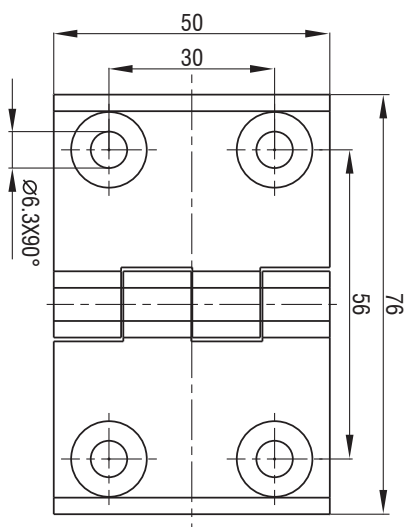
M6 沉头螺钉固定 Countersunk Screw M6
